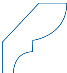
Bed Mould 1/2" x 1-5/8" Projection 1-1/8" Drop 1-1/4"
