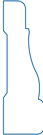
356 Casing 11/16" x 2-1/4"
